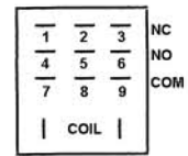
RY1, RY2 PINOUT
