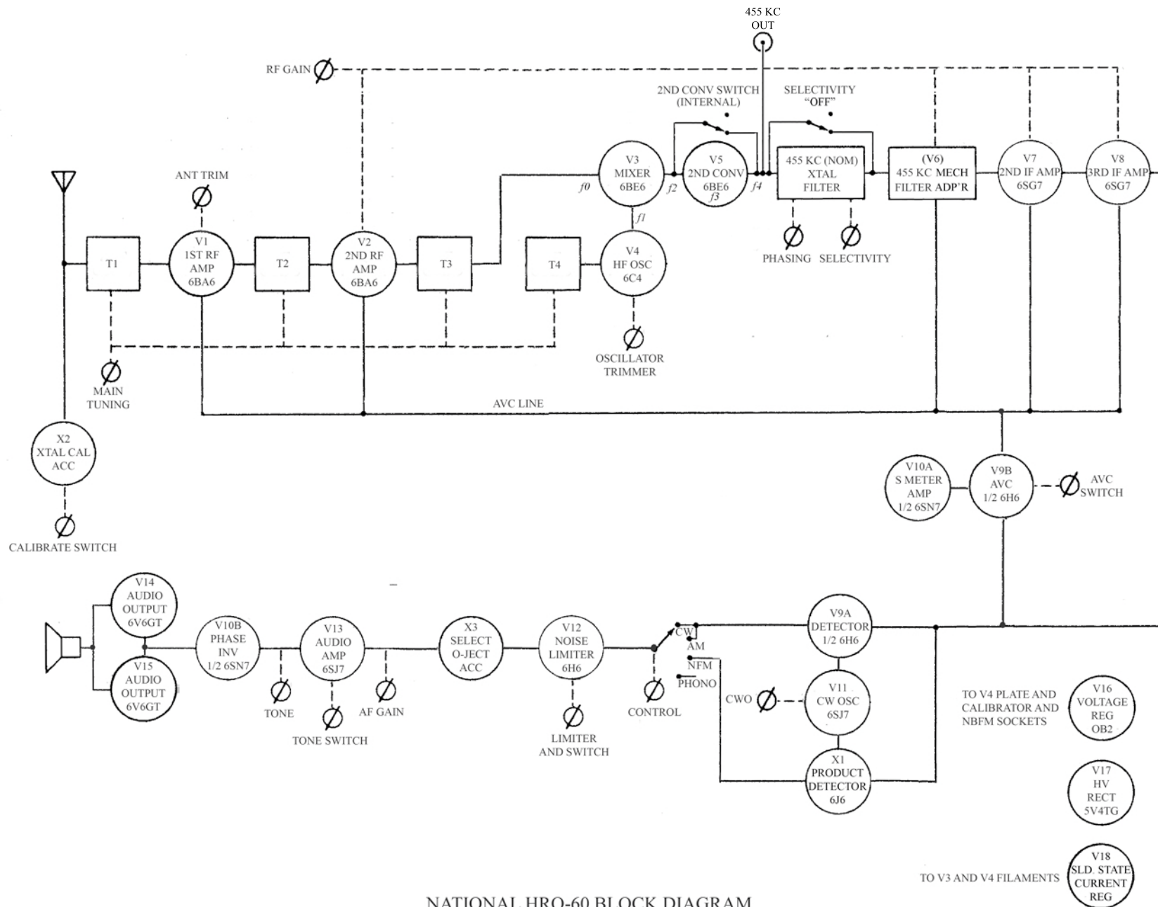
NATIONAL HRO-60 BLOCK DIAGRAM AS MODIFIED IN S/N 345-1003
